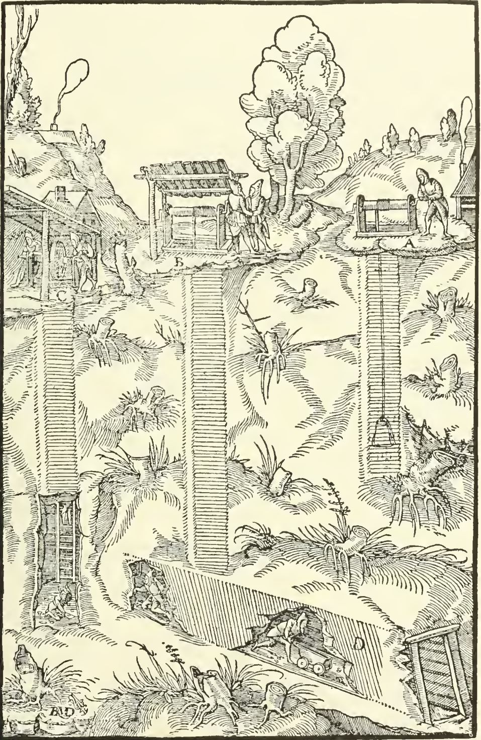
THREE VERTICAL SHAFTS, OF WHICH THE FIRST, A, DOES NOT REACH THE TUNNEL ; THE SECOND, B, REACHES THE TUNNEL ; TO THE THIRD, C, THE TUNNEL HAS NOT YET BEEN DRIVEN. D—TUNNEL.
